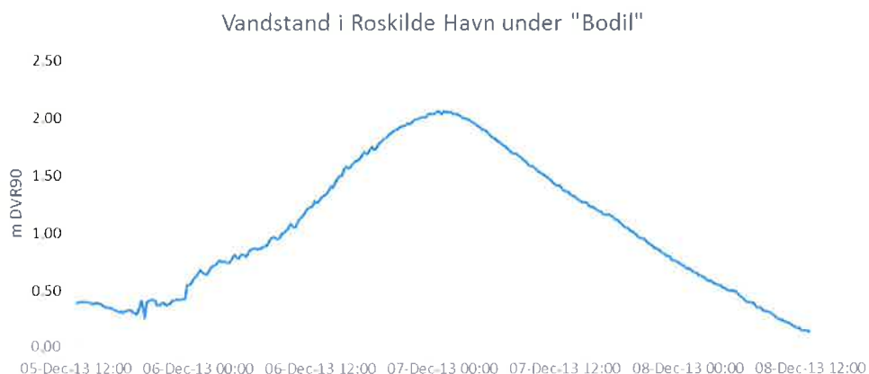
Figur 2 Vandstand i Roskilde Havn under Bodil i december 2013. Kilde: /2/
