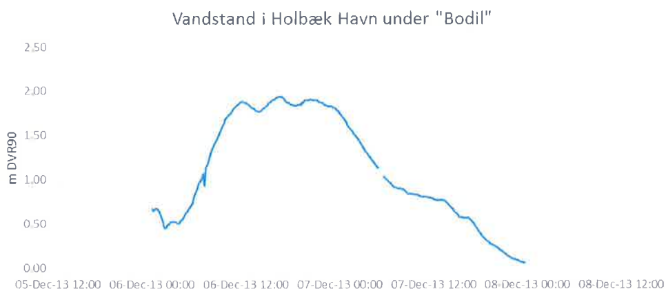
Figur 3 Vandstand i Holbæk Havn under Bodil i december 2013. Kilde: /2/
